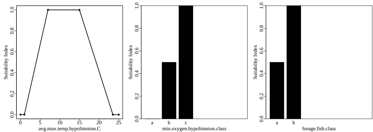
Figure 1. Suitability index graphs for variables included in the laketroutStocked model in ecorest .
