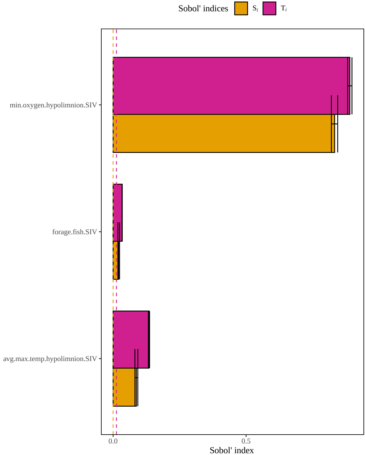
Figure 5. Results of a sensitivity analysis for the laketroutStocked model based on a geometric mean structure. Dashed lines represent baseline numerical approximation error for S_i and T_i ( i.e. , dummy variables).
