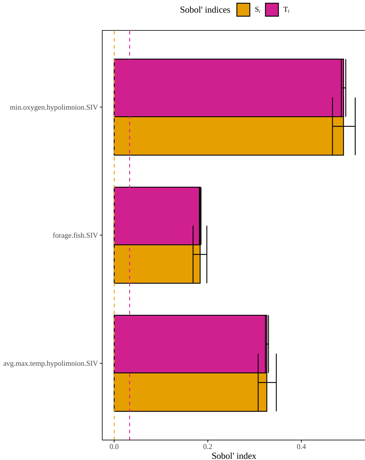
Figure 4. Results of a sensitivity analysis for the laketroutStocked model based on an arithmetic mean structure. Dashed lines represent baseline numerical approximation error for S_i and T_i ( i.e. , dummy variables).
